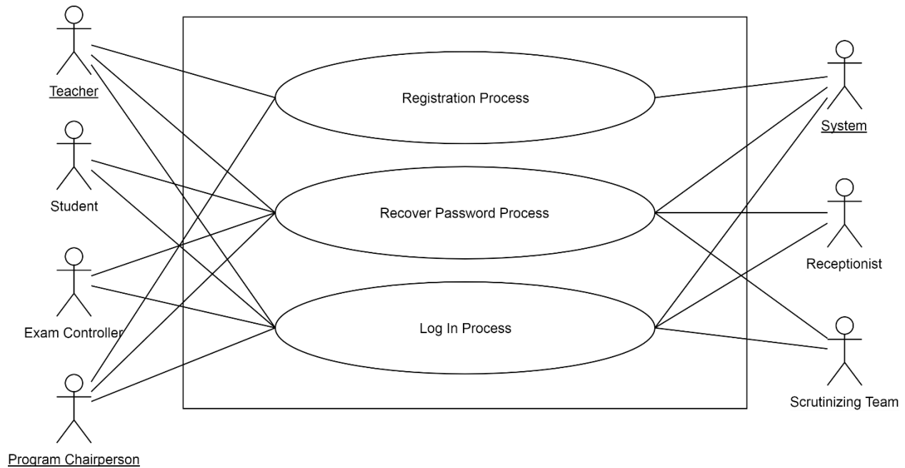
Figure 1: Usecase Level-1.1-Authentication
