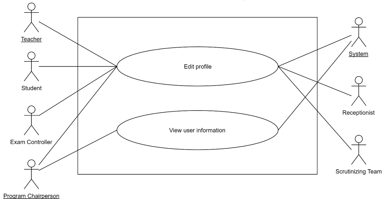
Figure 4: Usecase level-1.4-Profile management
