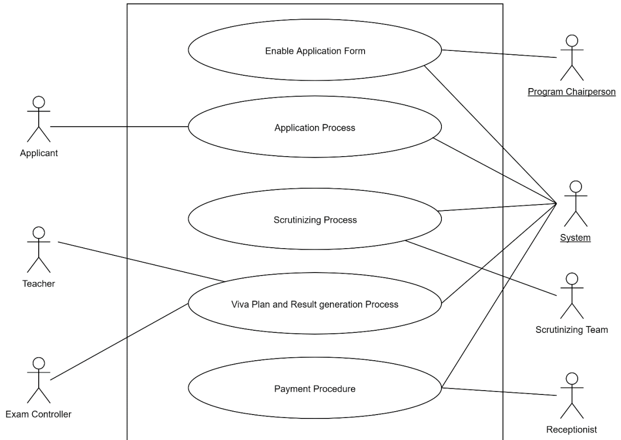
Figure 5: Usecase Level-1.2- Admission System
