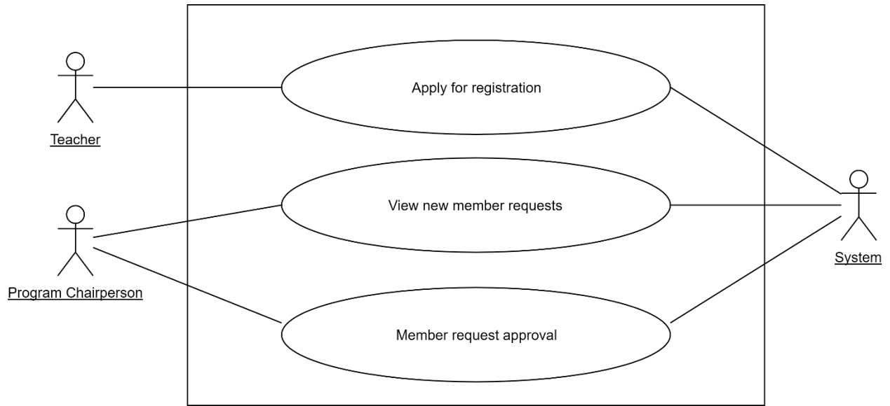
Figure 2: Usecase Level-1.1.1-Registration process
