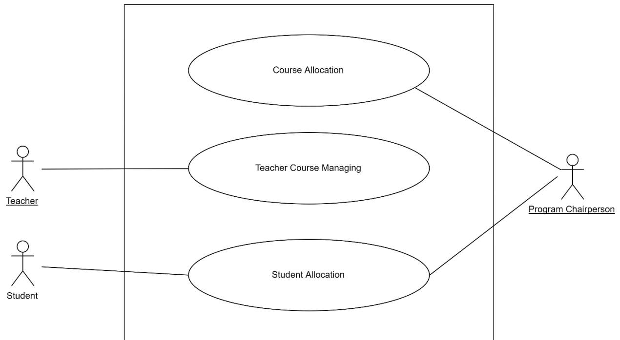
Figure 6: Usecase Level-1.3-Result generation system
