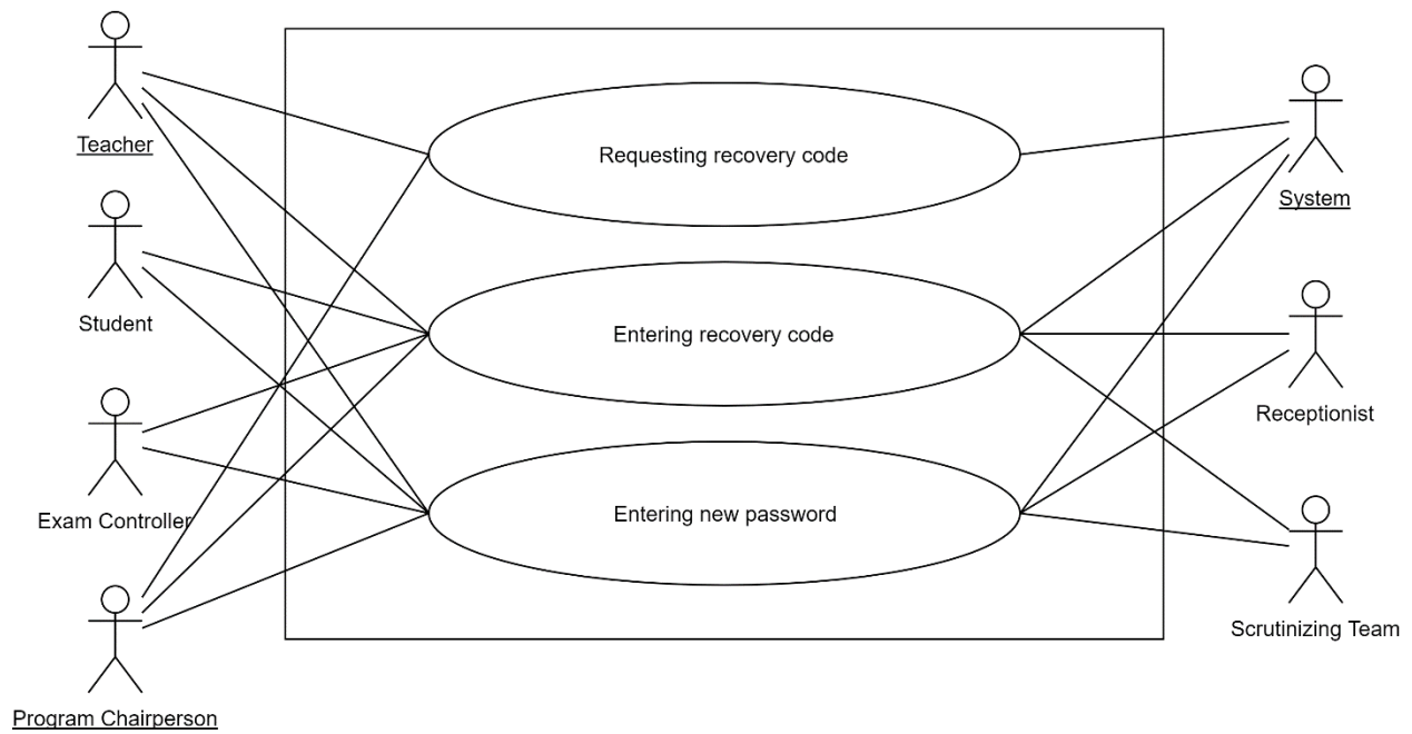
Figure 3: Usecase Level-1.1.2-Recover password process
